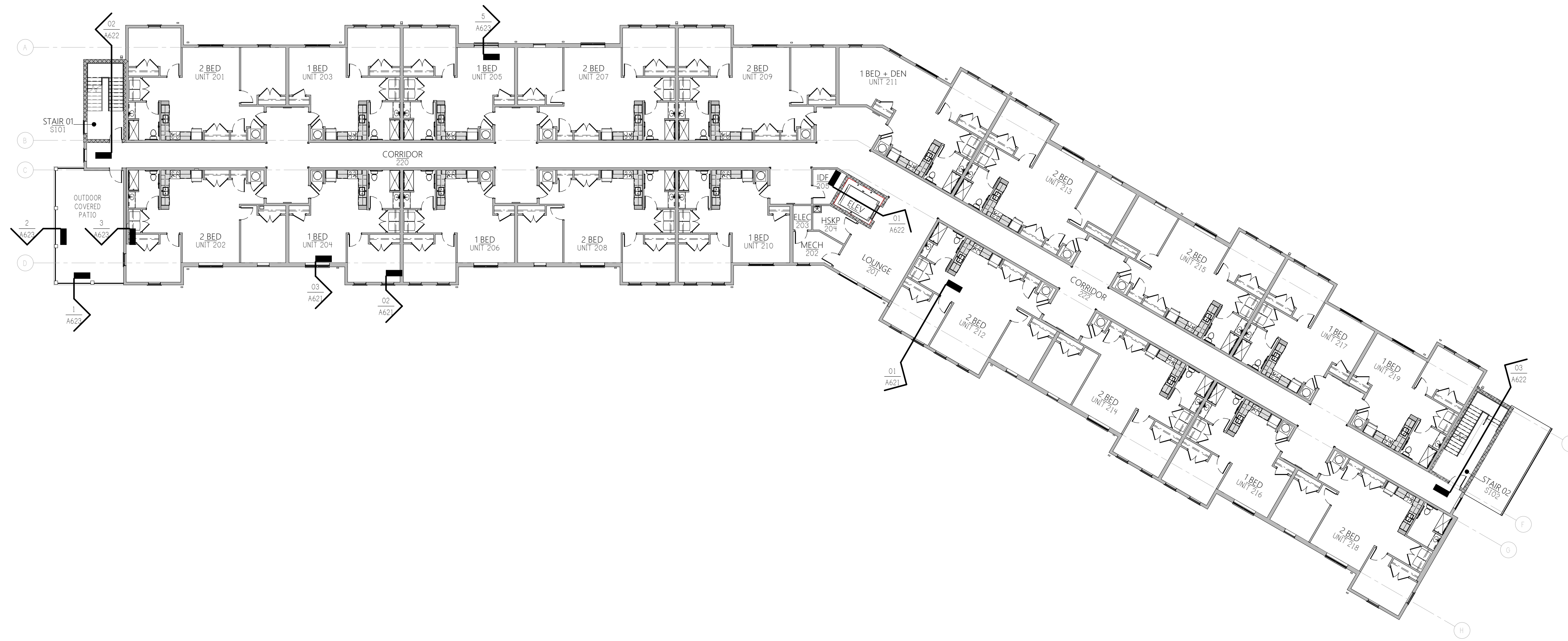
COMPOSITE SECOND FLOOR PLAN
