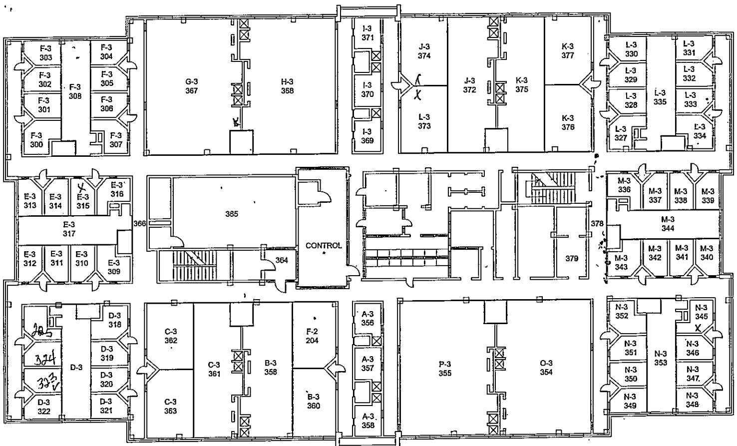
3 THIRD FLOOR PLAN
