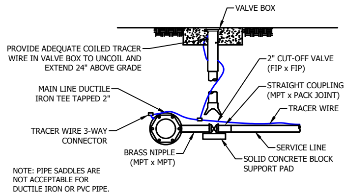
2 C2.3 2" CUT-OFF VALVE FOR SERVICE LINES DUCTILE IRON OR PVC MAIN LINE NOT TO SCALE
