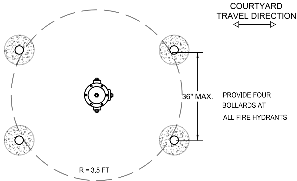
TYPICAL BOLLARD SETTING PLAN
