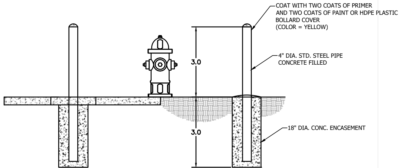
1 BOLLARD DETAIL C2.2 NOT TO SCALE
