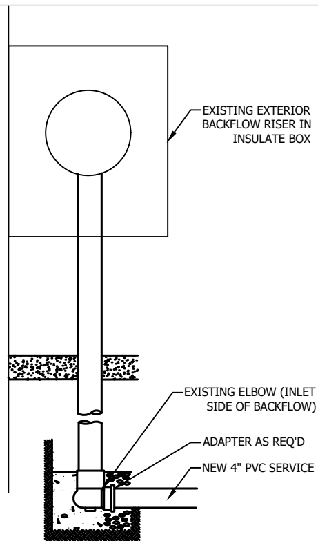
3 C2.3 SERVICE CONNECTION FOR EXTERIOR BACKFLOW DEVICE NOT TO SCALE
