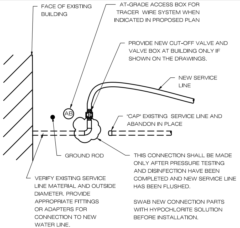
4 C2.1 CONNECTION OF NEW SERVICE LINE TO EXISTING BUILDING SERVICE LINE (TYPICAL) NOT TO SCALE
