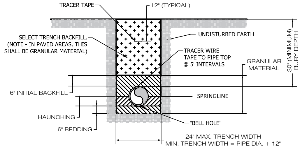
1 C2.1 TYPICAL SECTION - PIPE BEDDING AND INITIAL BACKFILL FOR PVC AND HDPE PIPE NOT TO SCALE
