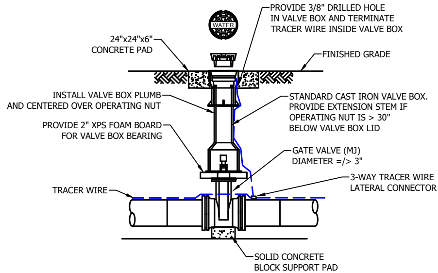
1 C2.3 CUT-OFF VALVE & VALVE BOX DETAIL - MAIN LINES NOT TO SCALE
