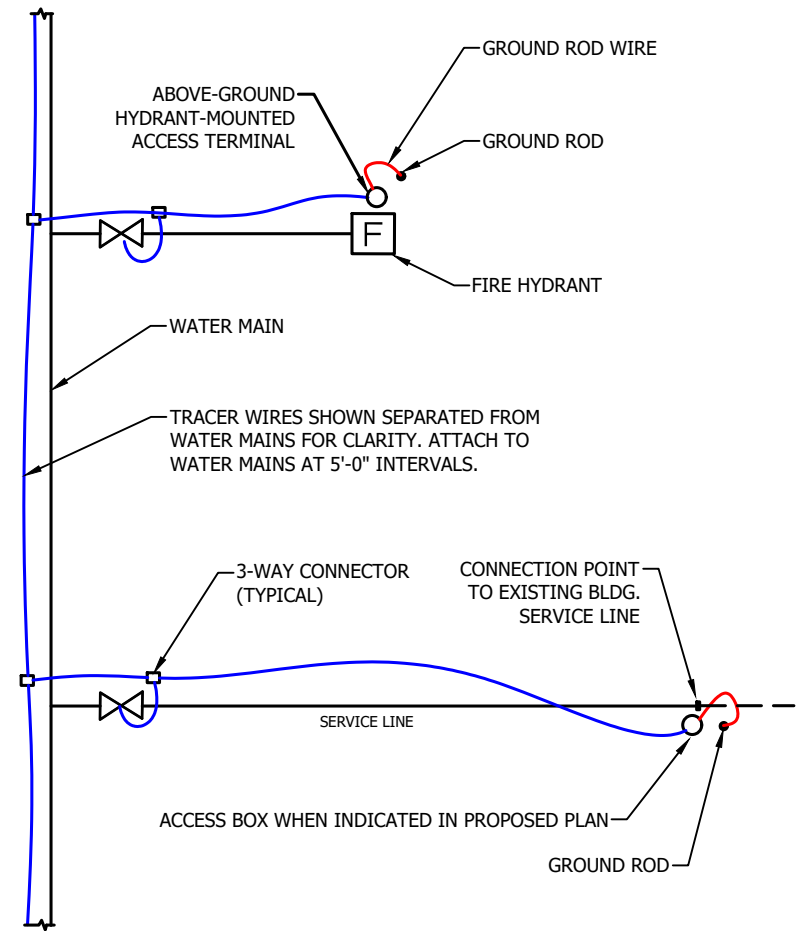
3 C2.1 TRACER WIRE SCHEMATIC NOT TO SCALE
