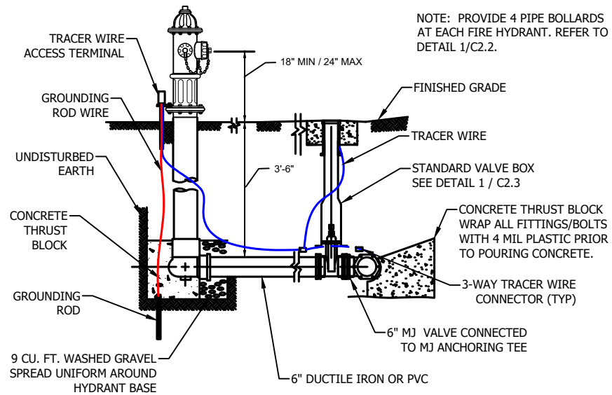
2 FIRE HYDRANT & VALVE BOX DETAIL C2.2 NOT TO SCALE
